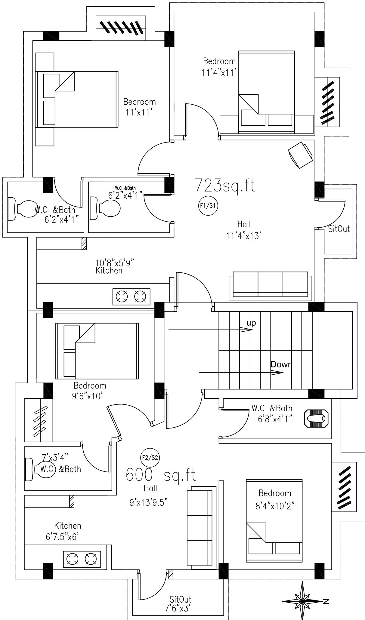
Typical First and Second FloorFirst Floor
