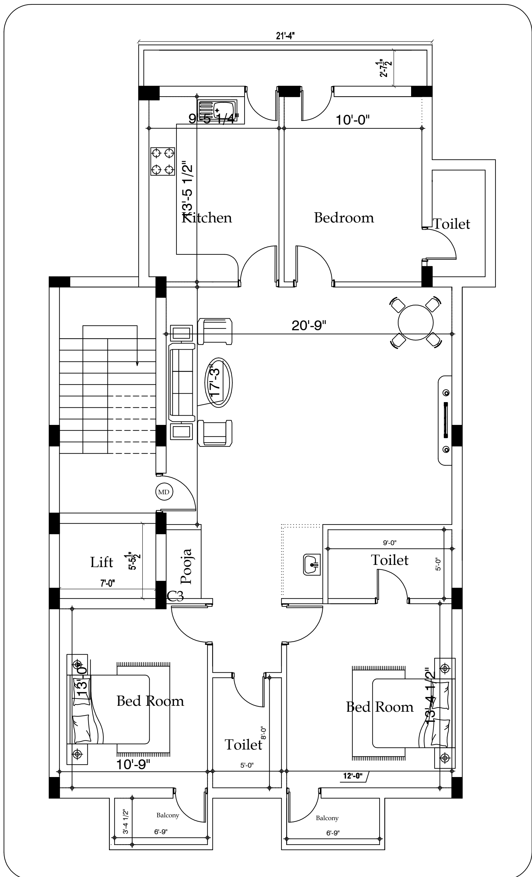
Typical Floor plan (1745 sq.ft)
